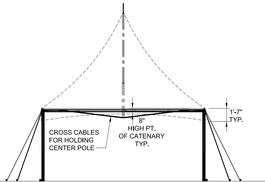
END VIEW
