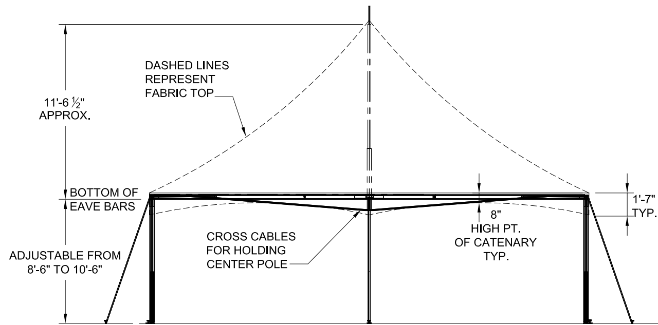
SIDE VIEW
