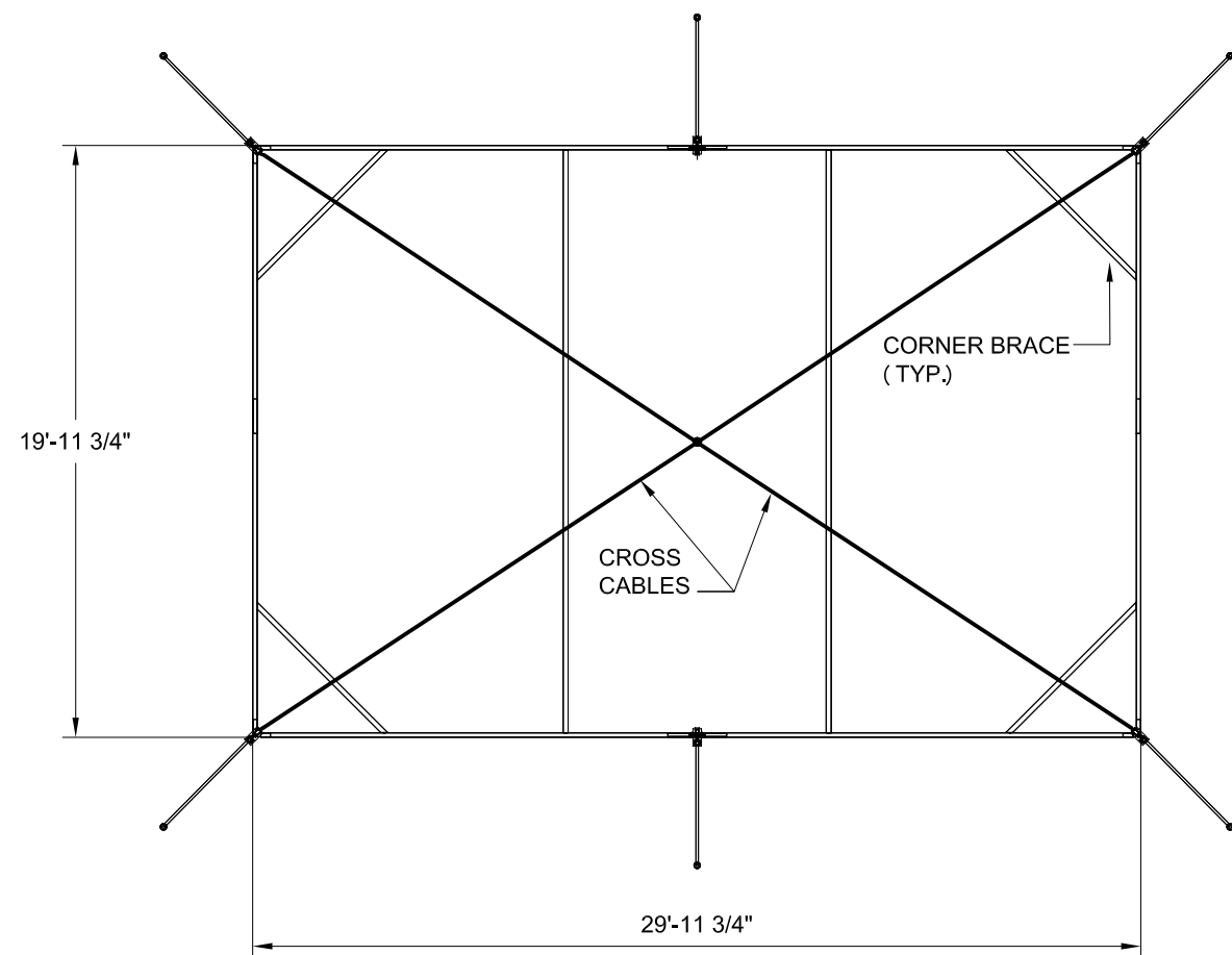
PLAN VIEW
