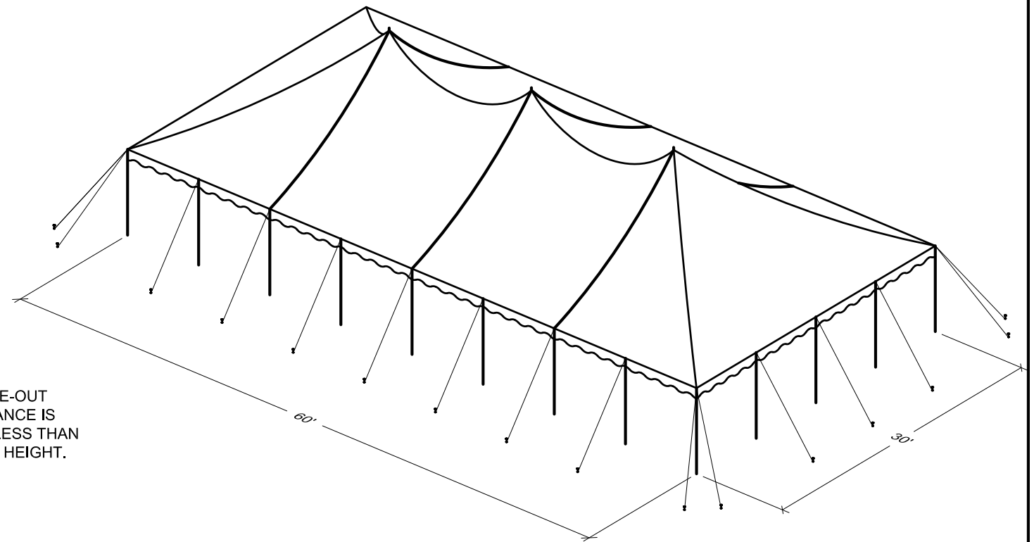
ISOMETRIC
