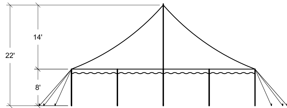
SIDE ELEVATION
