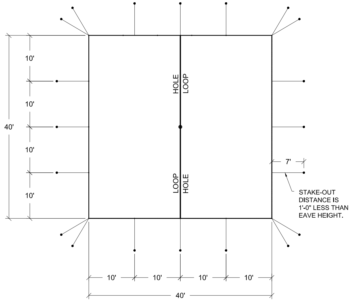
PLAN (2) ENDS
