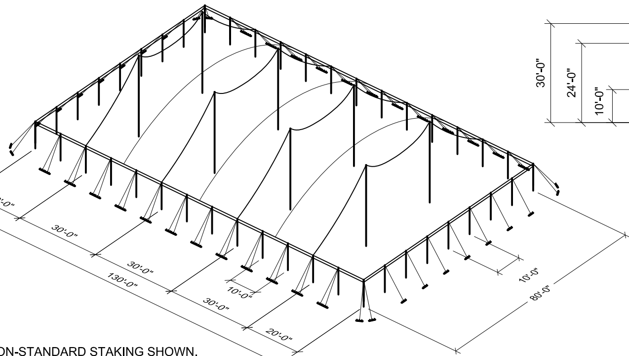
ISOMETRIC
