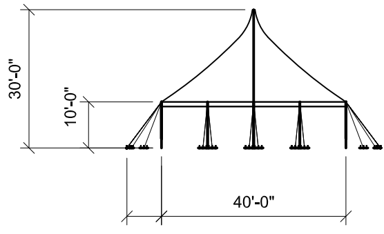
SIDE ELEVATION SCALE: 1" = 30'
