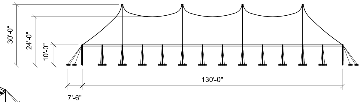
SIDE ELEVATION
