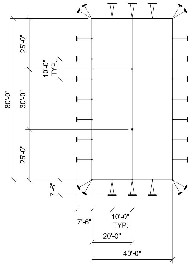
PLAN
