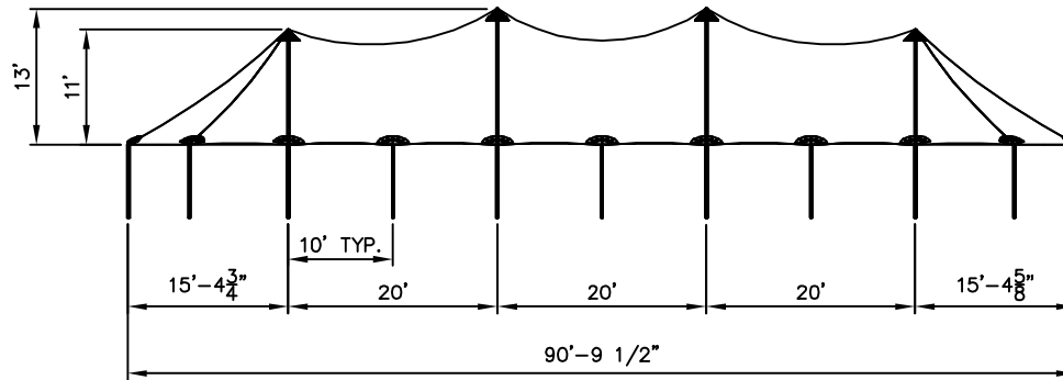
SIDE VIEW
