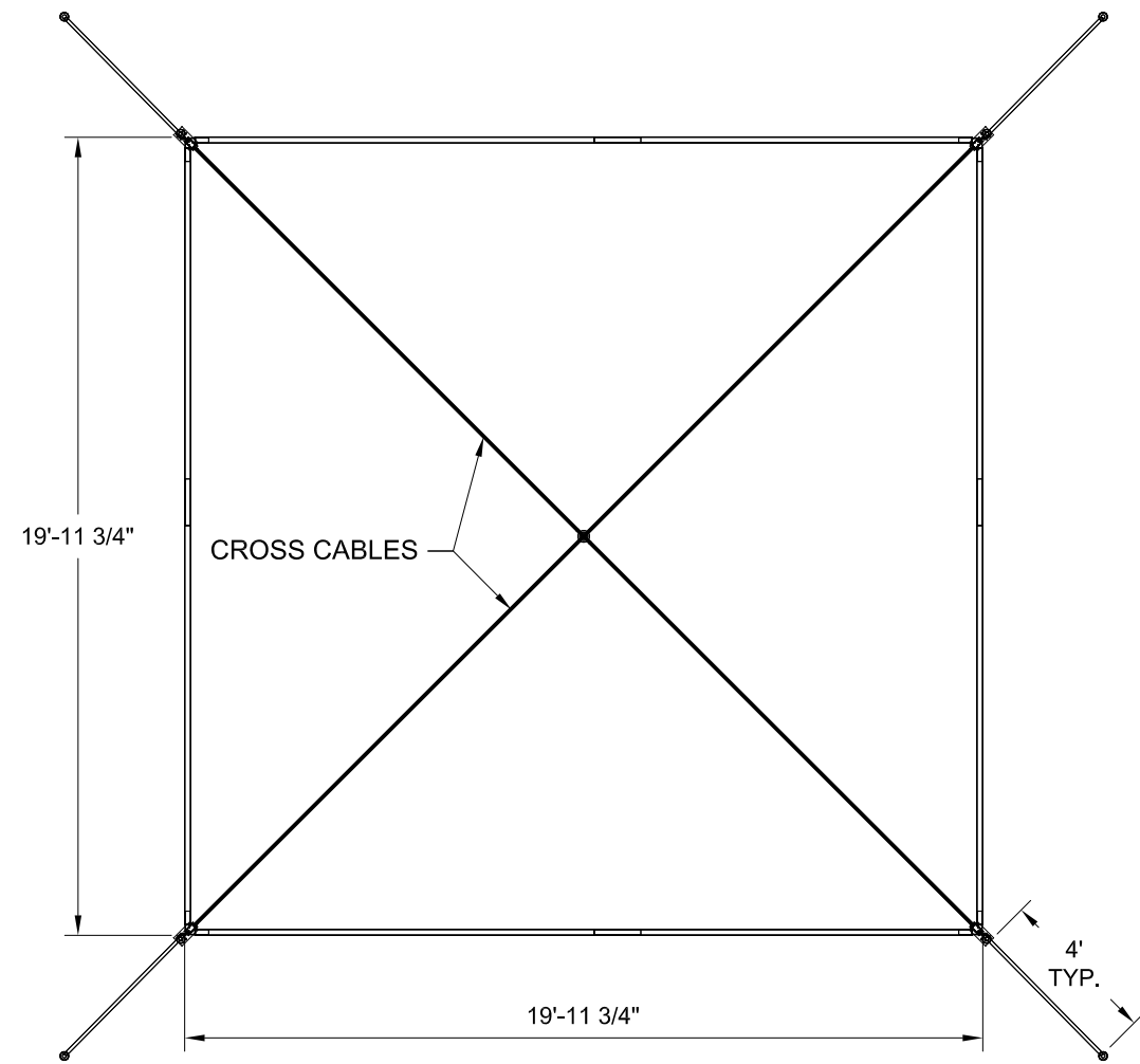
PLAN VIEW
