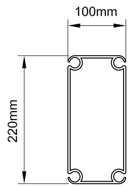
BEAM PROFILE RAFTERS & SIDE UPRIGHTS
